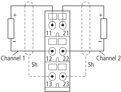
XN-S3...-SSB for XN-2A0-I(0/4...20MA)
