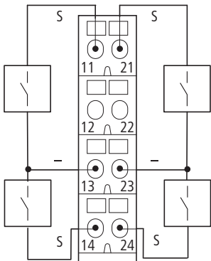
XN-S4...-SBBS for XN-4DI-24VDC-N
