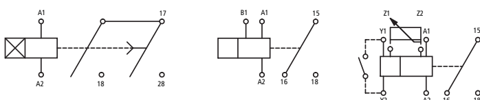
ON-DELAYED
