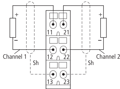
XN-S3...-SSB for XN-2A0-U(-10/0...+10VDC)
