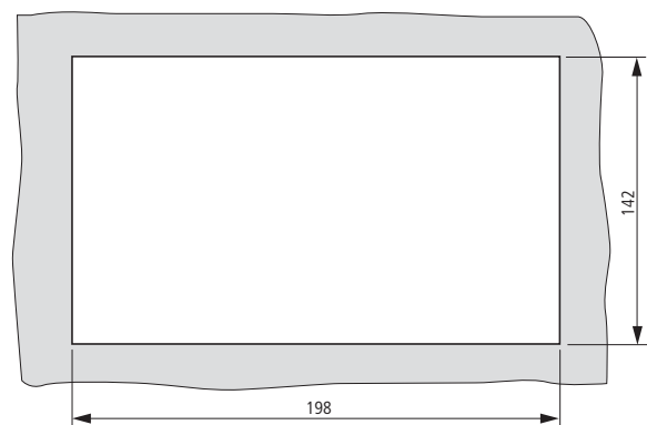
Mounting dimensions
