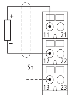
XN-S3...-SSB for XN-1A0-I(0/4...20MA)
