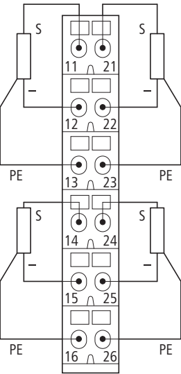
XN-B6...-SBCSBC for XN-32DO-24VDC-0.5A-P
